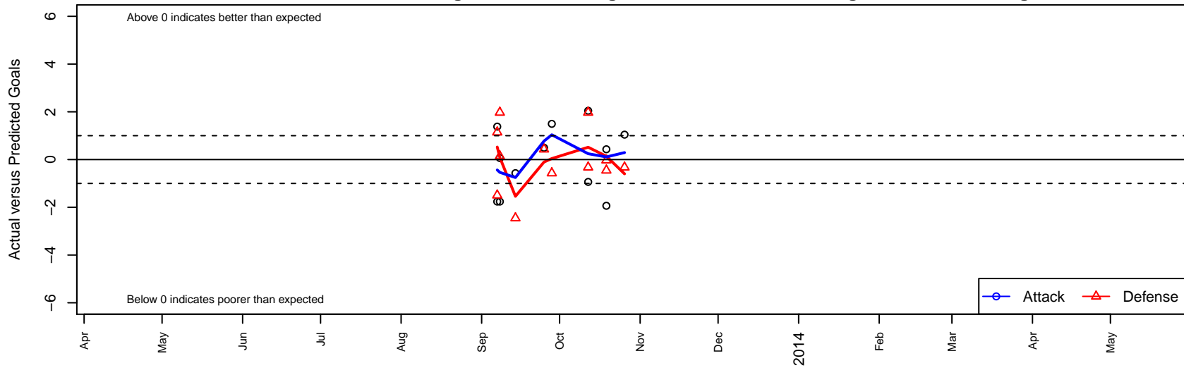
Pullman Pumas BU16-18 Tattershall B95 Dots are actual minus expected GF (blue circles) and GA (red triangles). Blue line is smoothed change in attack strength. Red is smoothed change in defense strength.
